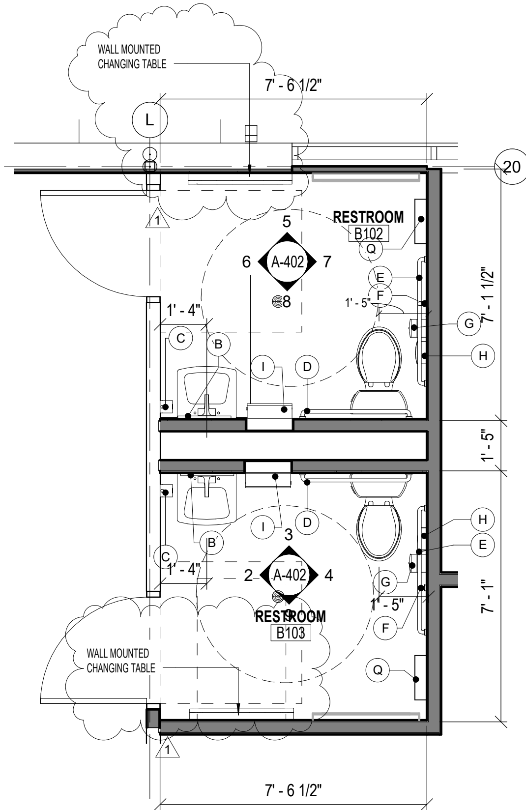
1 ENLARGED TOILET ROOM FLOOR PLANS ASK-02 SCALE: 3/8" = 1'-0"
