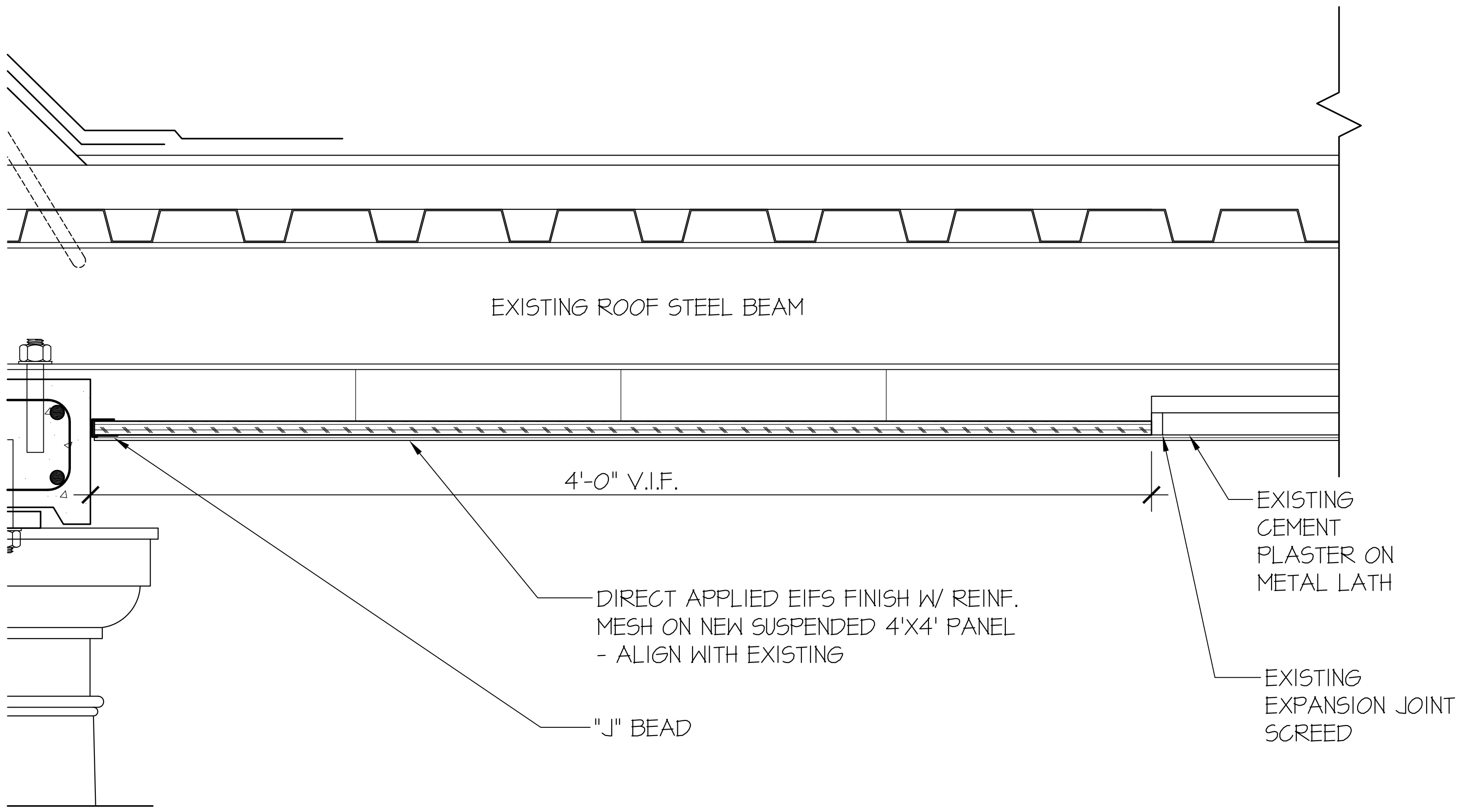
CEILING PANEL DETAIL SCALE: 3"=1'-0"
