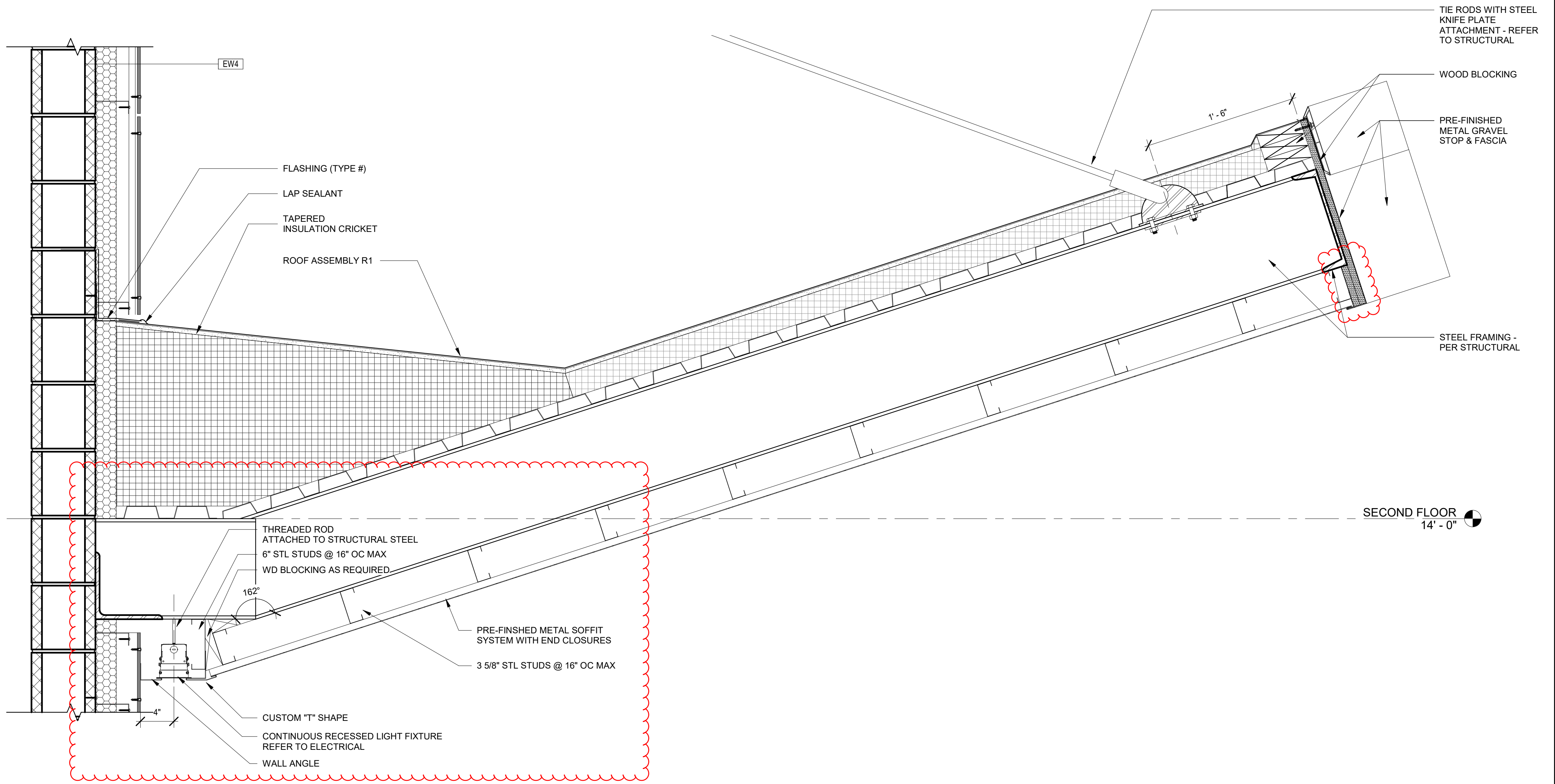
A1 VERTICAL DETAIL - SLOPED CANOPY - LONGITUDINAL SECTION 1 1/2" = 1'-0"
