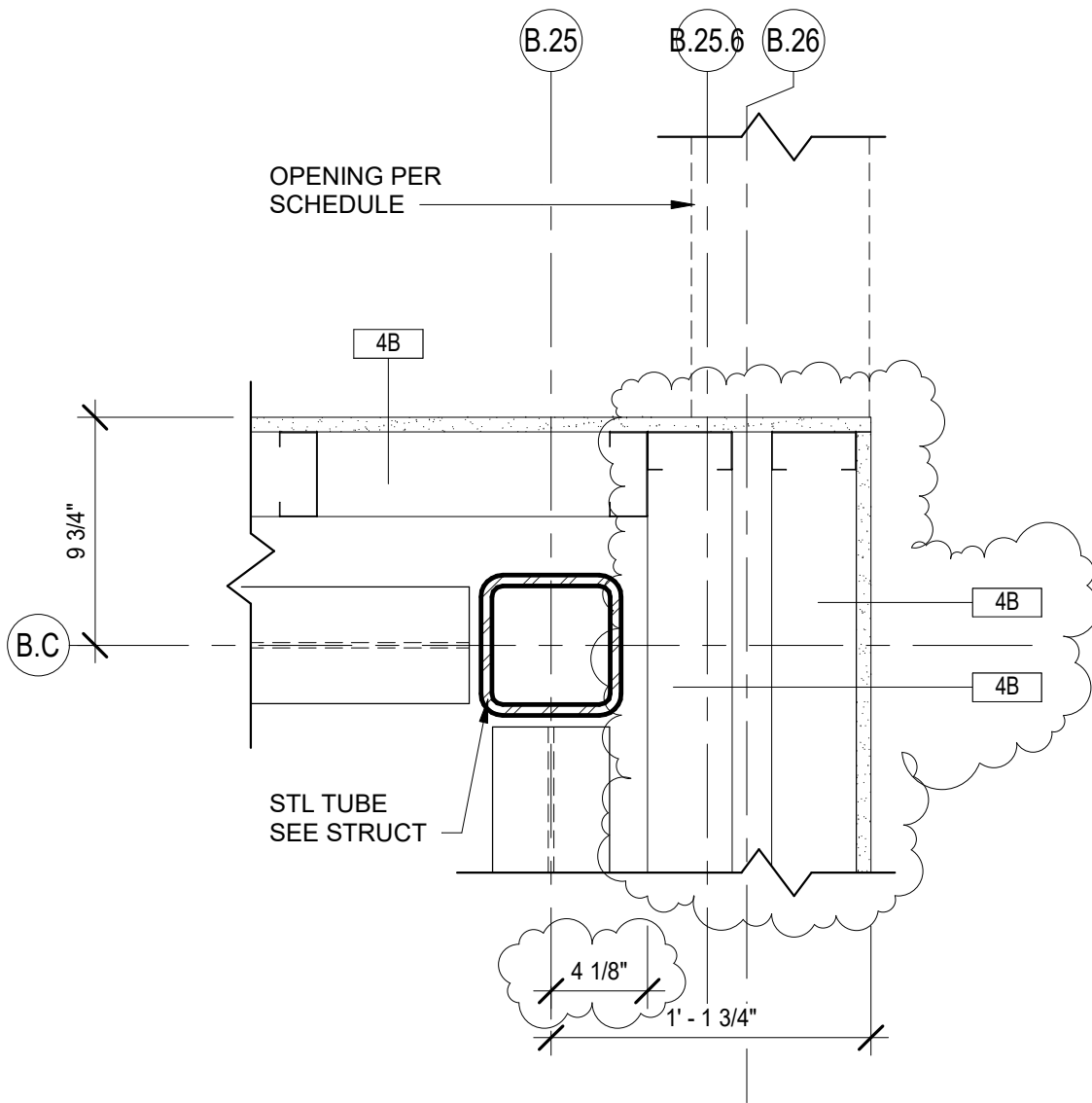
A6 ENLARGED PLAN DETAIL 1 1/2" = 1'-0"
