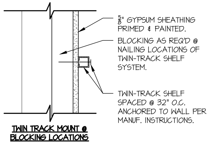
2 TRACK MOUNTING DETAILS SCALE : 3" = 1'-0"
