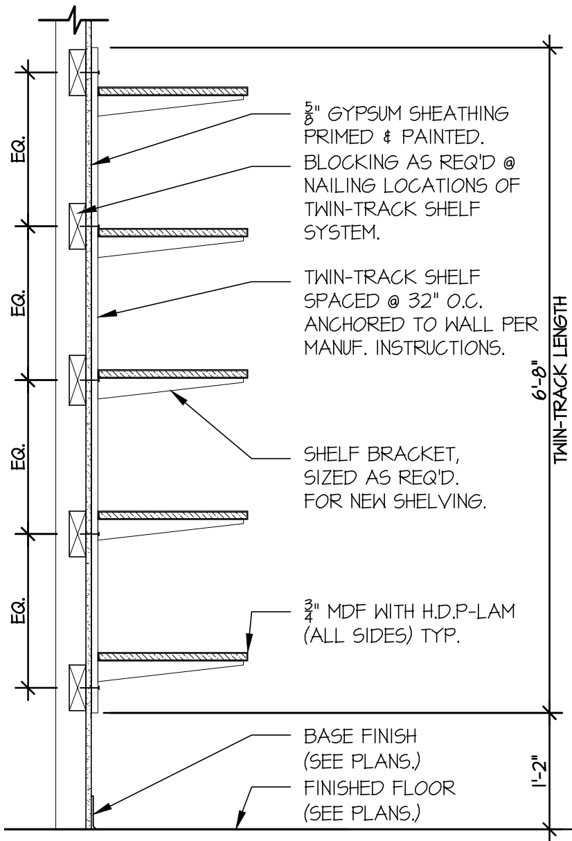
1 ADJUSTABLE SHELVING SECTION SCALE : 3/4" = 1'-0"
