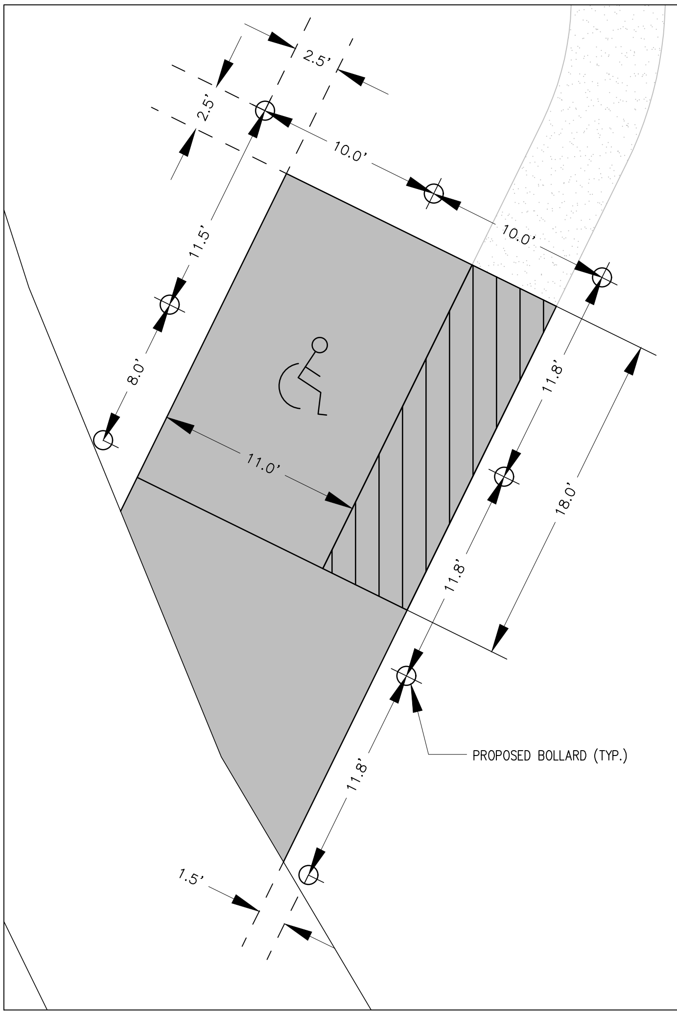
DETAIL: BOLLARD SPACING
